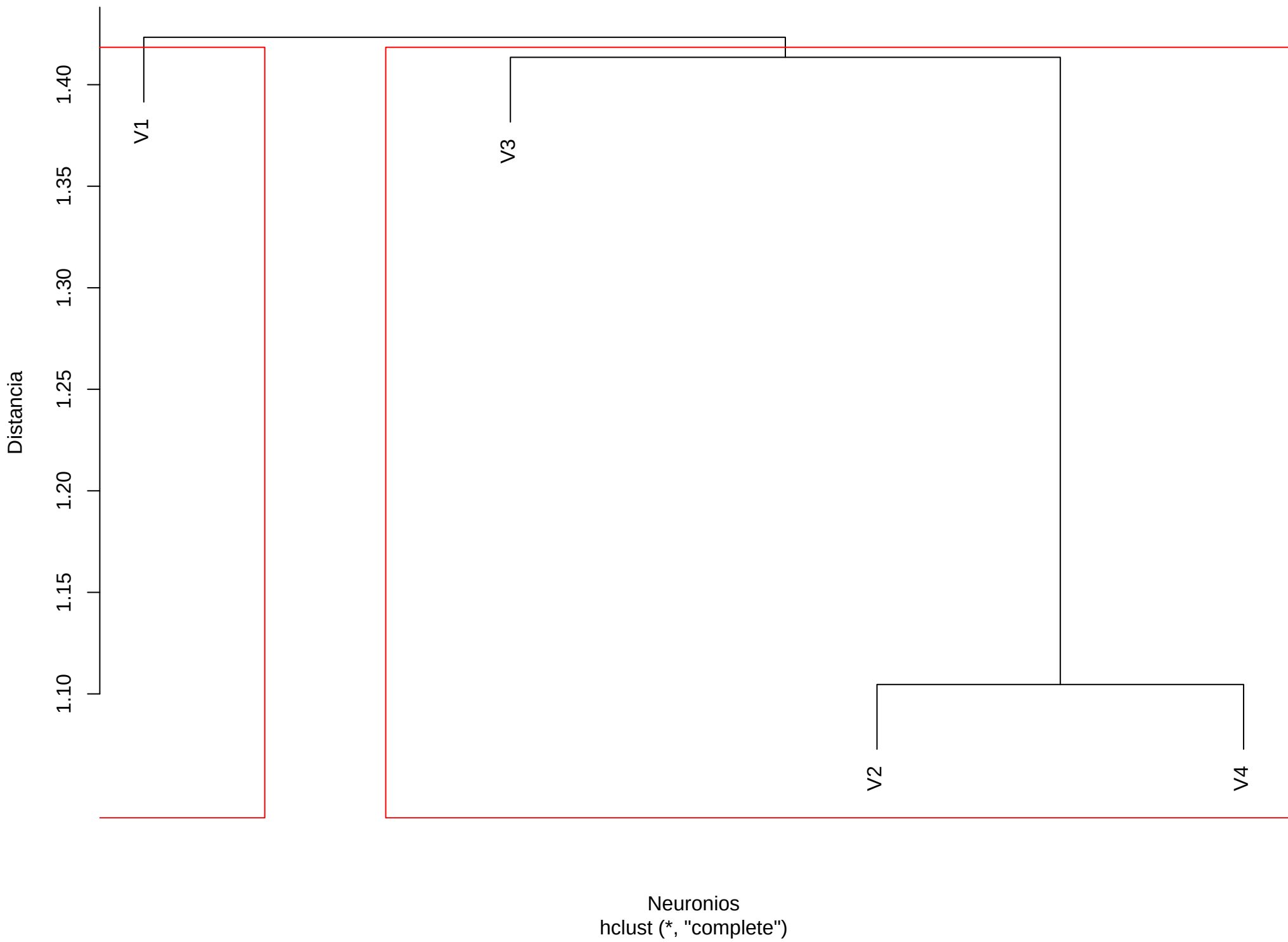
Dendrograma (k=2) | scene | bubble | Fold 2
