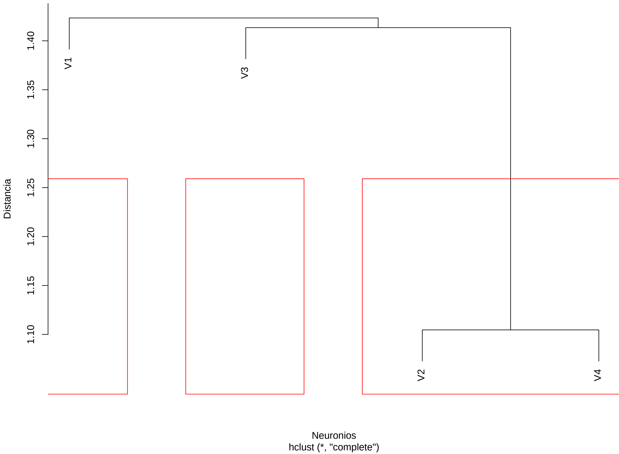
Dendrograma (k=3) | scene | bubble | Fold 2
