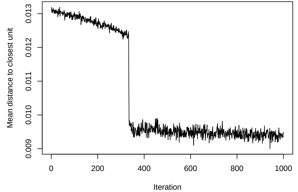
Codebook – Segments
