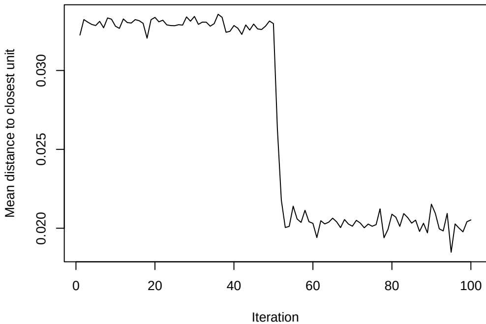
Codebook – Segments
