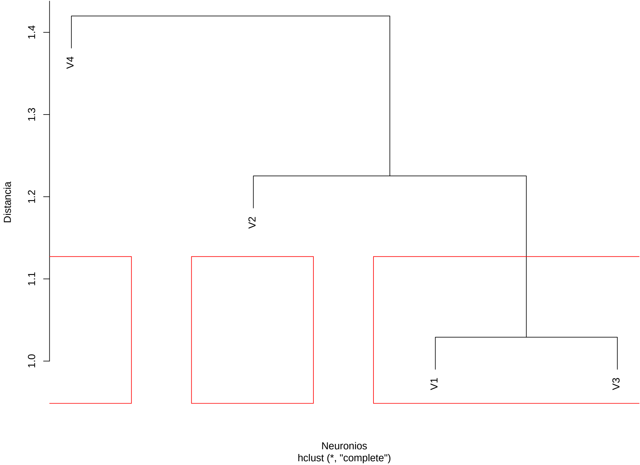
Dendrograma (k=3) | scene | bubble | Fold 1
