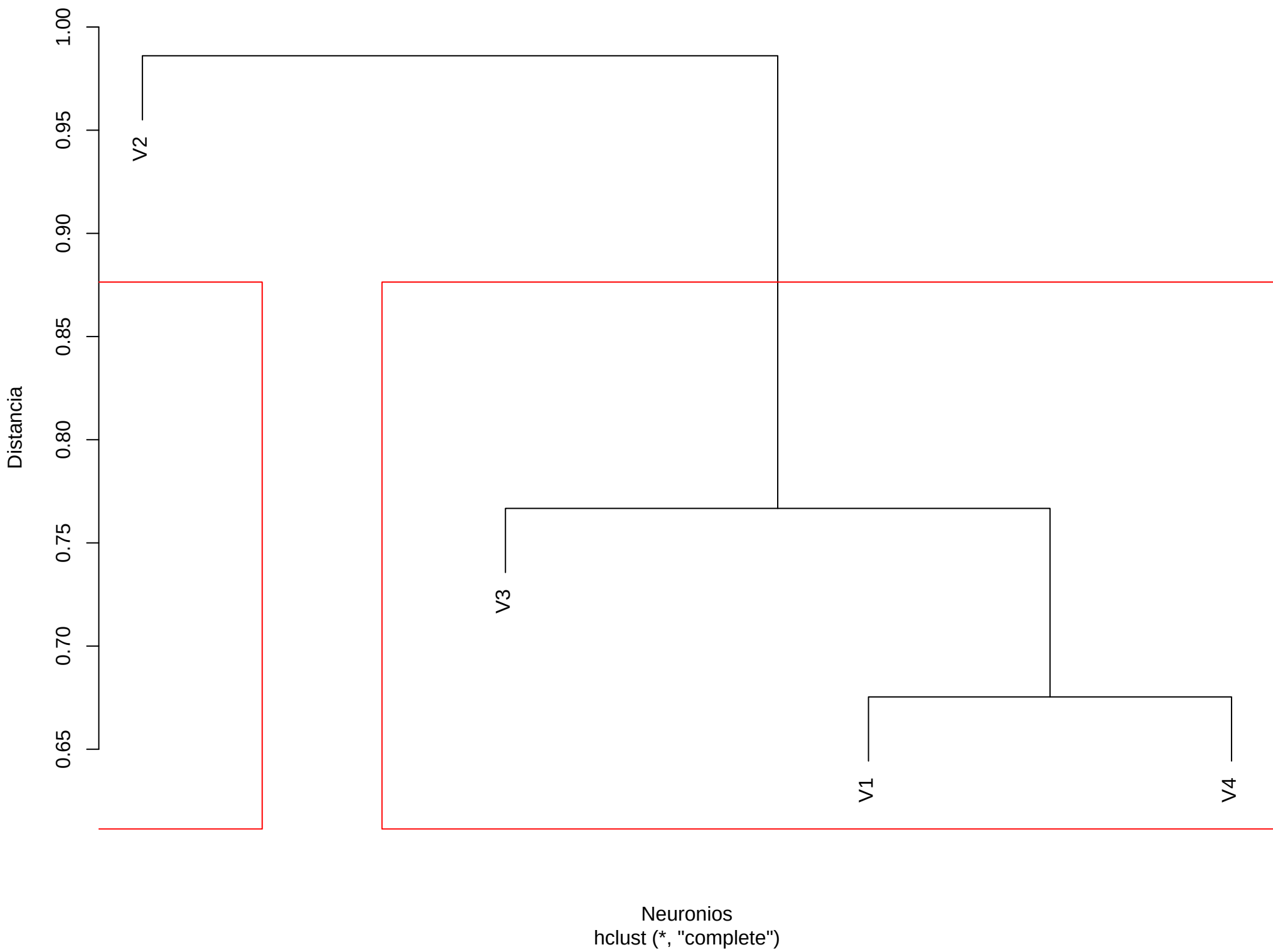
Dendrograma (k=2) | scene | gaussian | Fold 3
