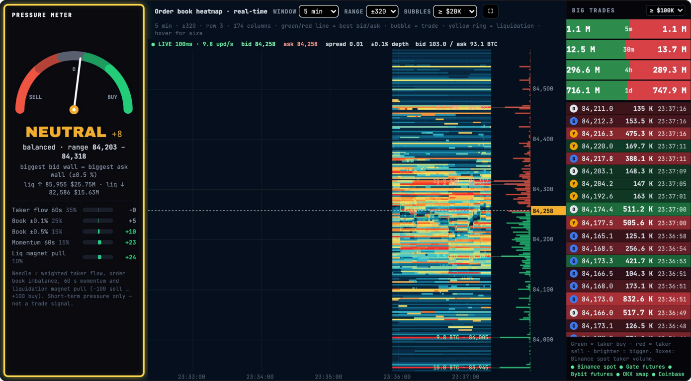
Pressure meter · order book heatmap · big trades.
