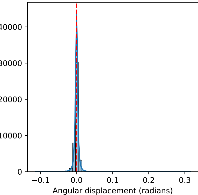
Distribution of angular displacements
