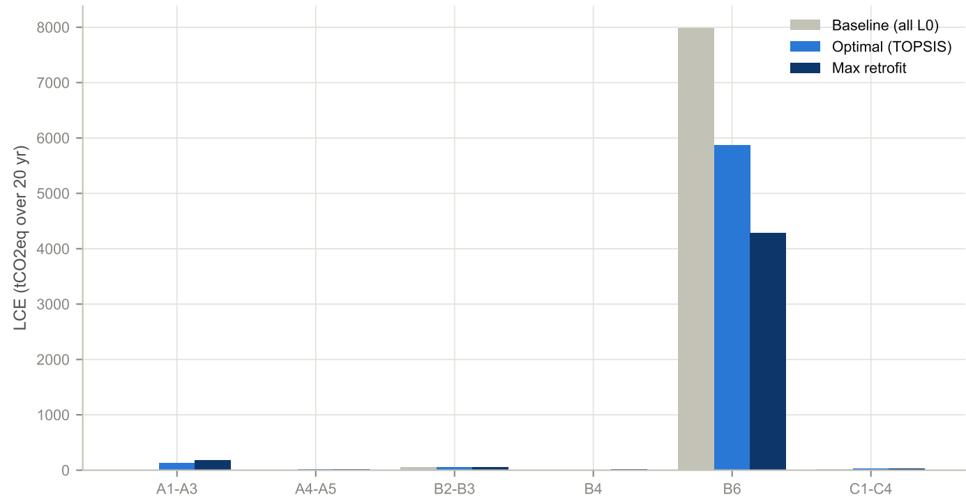
Embodied vs operational carbon across retrofit depth (NZEB paradox)
