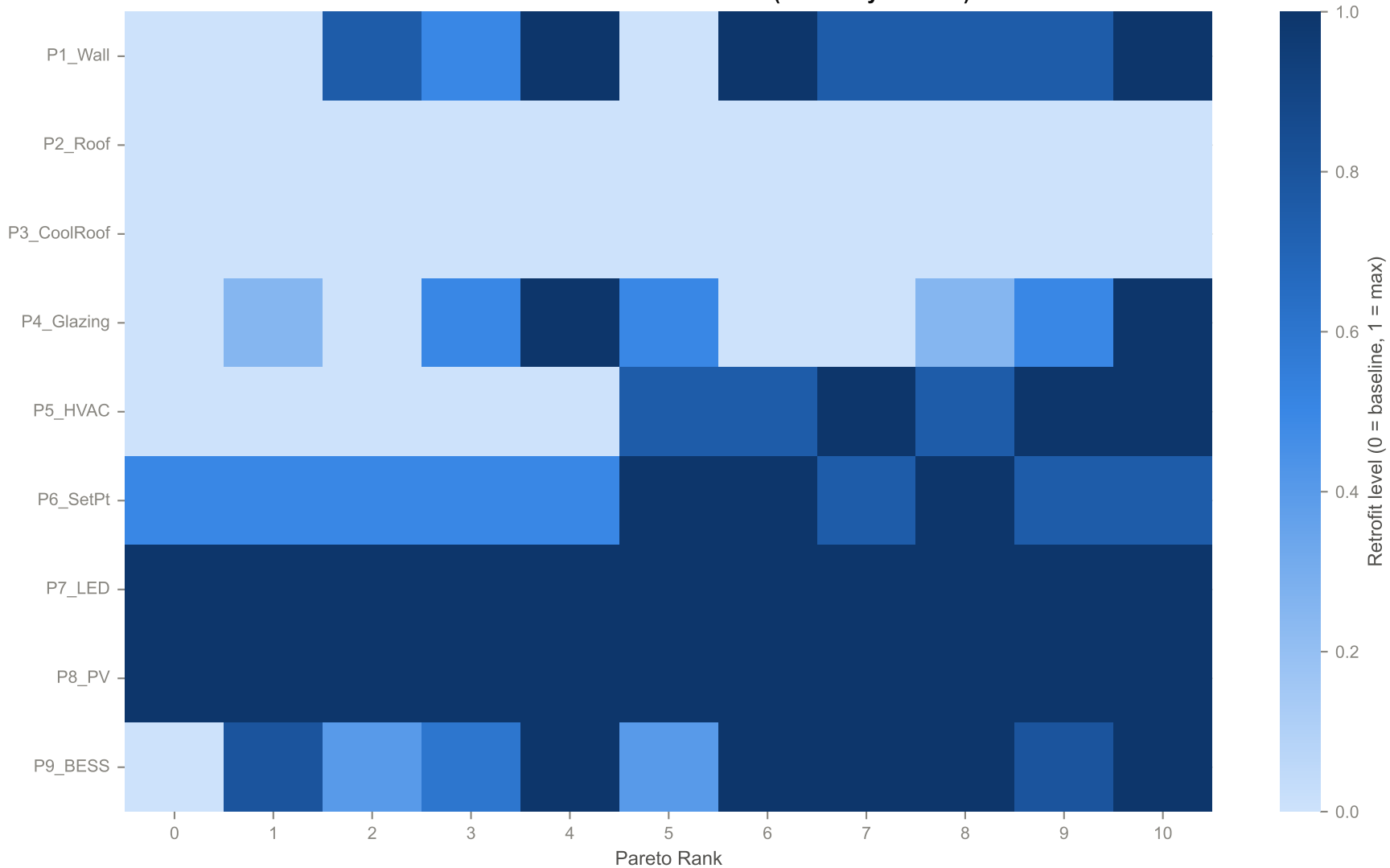
Renovation Levels for Pareto Solutions (Sorted by TOPSIS)
