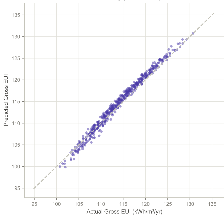
Linear Reg ( R^2 = 0.9695 )
