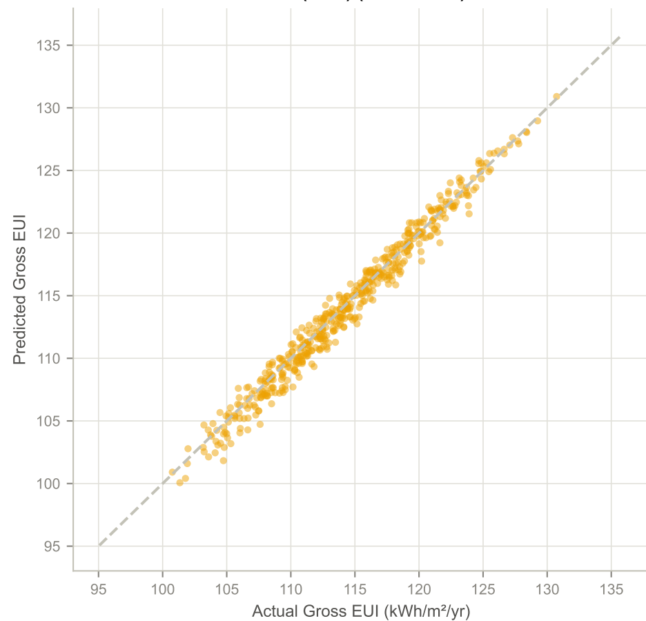
ANN (MLP) ( R^2 = 0.9744 )
