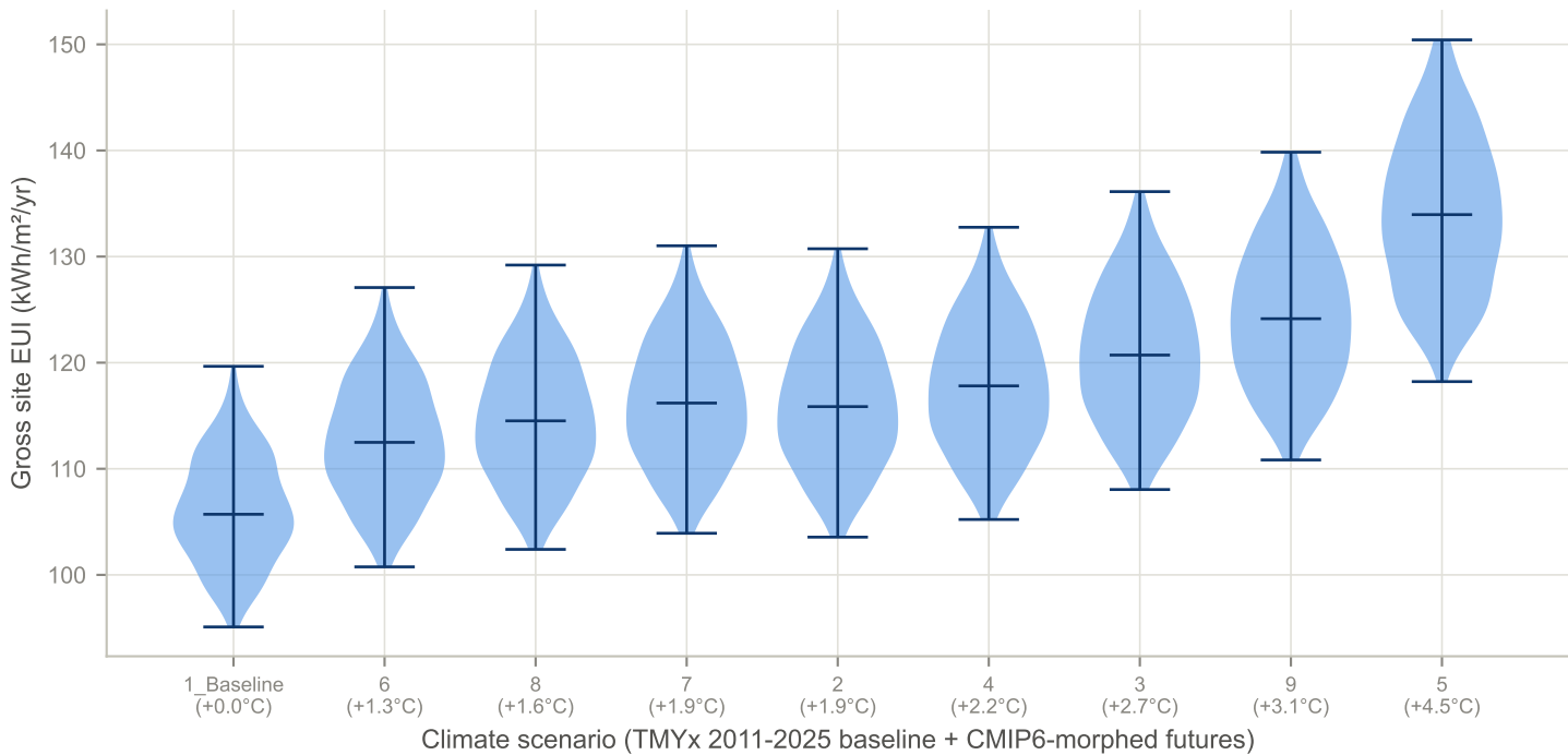
EUI distribution shifts under climate change (250 LHS runs per scenario)
