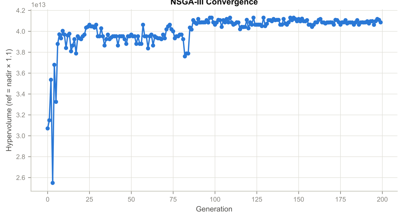
NSGA-III Convergence
