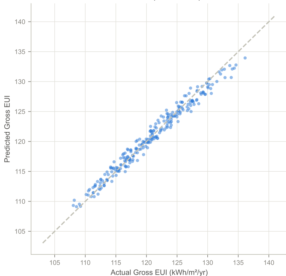
ANN (MLP) ( R^2 = 0.9656 )
