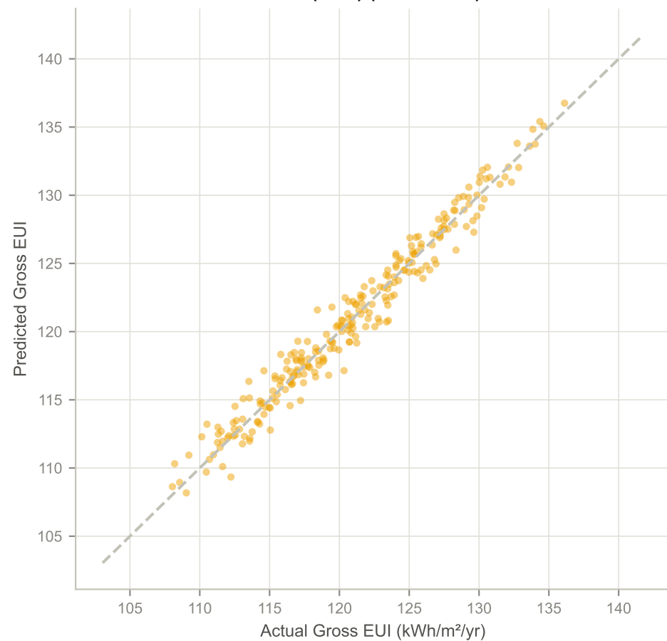
ANN (MLP) ( R^2 = 0.9652 )
