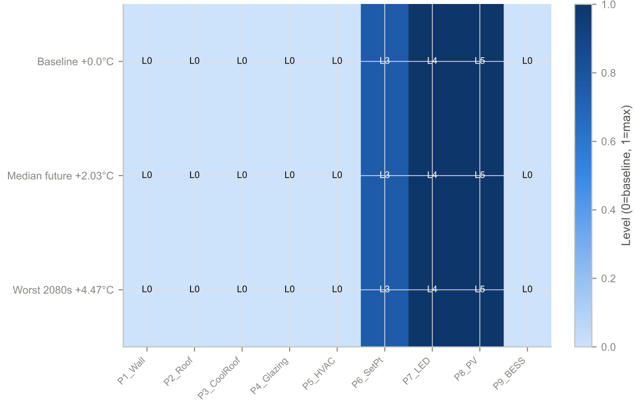
(b) Optimal package shifts with warming
