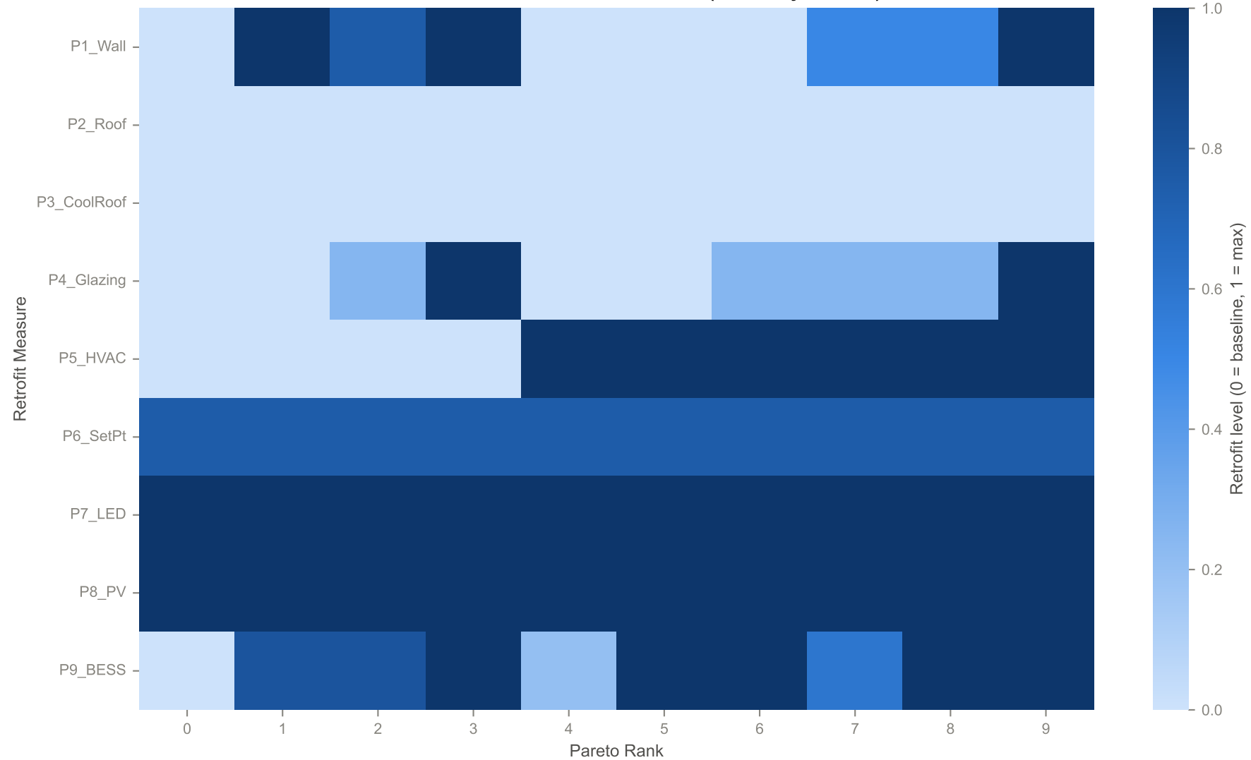
Renovation Levels for Pareto Solutions (Sorted by TOPSIS)
