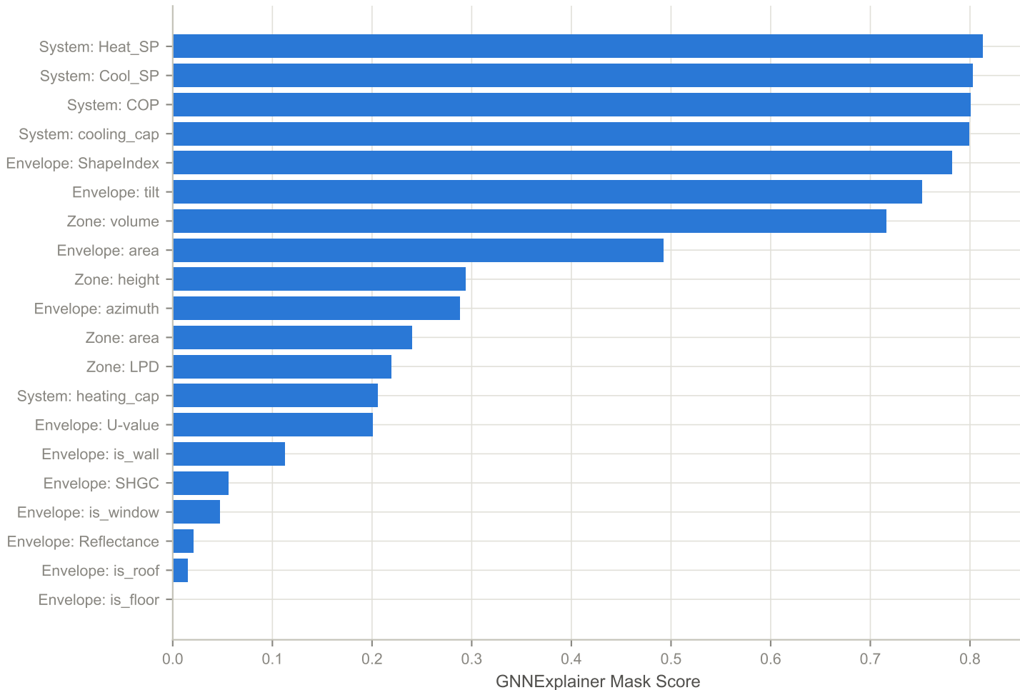
Feature Importance per Node Type
