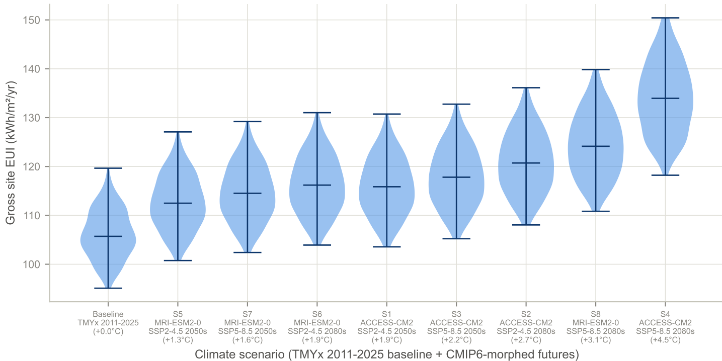
EUI distribution shifts under climate change (250 LHS runs per scenario)
