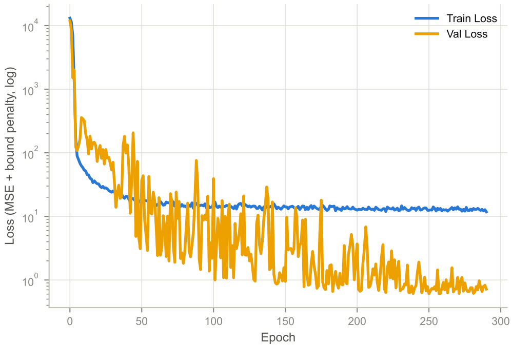
PI-HGAT Training Loss
