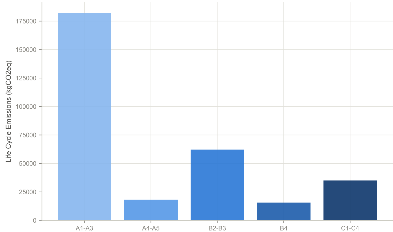
LCE Distribution by LCA Modules (Max Retrofit)
