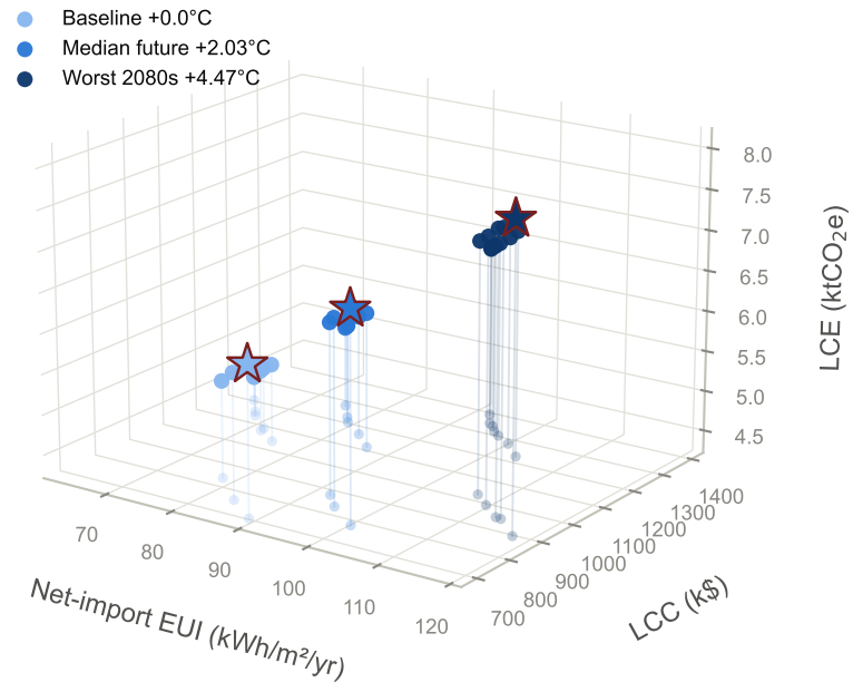
(a) Pareto fronts under warming: EUI × LCC × LCE (stars = TOPSIS best)
