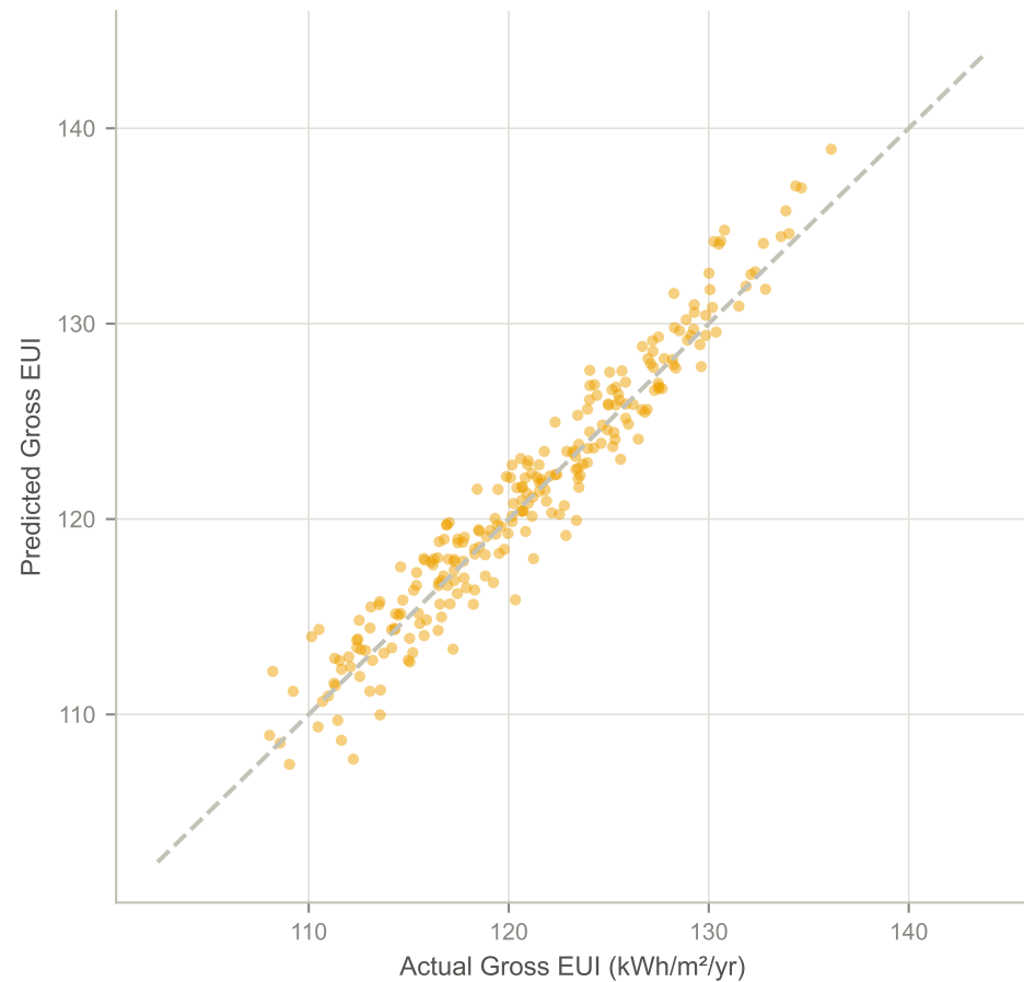
ANN (MLP) ( R^2 = 0.9287 )
