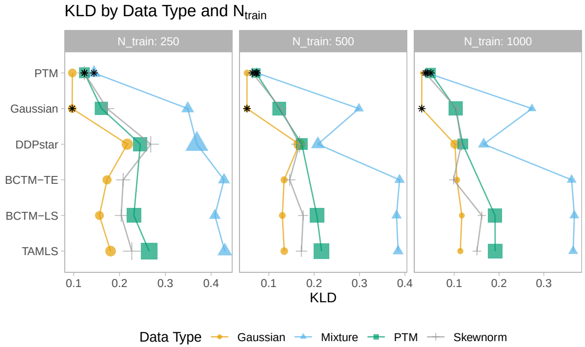
Figure I.2 Kullback-Leibler divergence. The plot shows the average of 100 replications with different seeds for pseudo-random number generation. The size of the point shapes is proportional to the standard deviation over these 100 replications. Within each panel and data type, a black star marks the best-performing observation.
