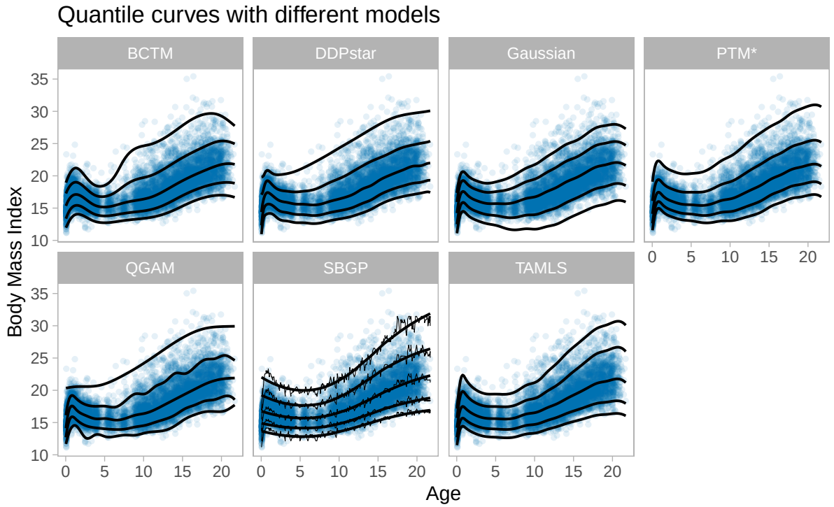
Figure J.2 Quantile curves at probability levels 0.01, 0.1, 0.5, 0.9, 0.99 for different models. The curves were produced with full-sample model runs. For SBGP, the available implementation returns posterior predictive samples at the specified age values rather than an analytic conditional quantile function. The SBGP curves shown here were therefore computed pointwise as empirical quantiles of 5,000 posterior predictive draws each for a grid of 150 values for age in [\min(\text{age}), \max(\text{age})] . Their local wiggleness reflects this sample-based reconstruction, including finite Monte Carlo variation and numerical inversion of the estimated transformation, and should not be interpreted as evidence for an intrinsic lack of smoothness. The overlaid smooth lines for SBGP are cubic regression splines applied only for visualization (using the ggplot2 default in geom_smooth ).
