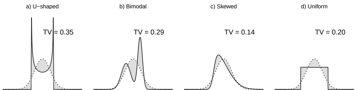
Figure D.1 Illustration of the total variation distance (TV) for four example densities. The total variation distance is the shaded area.
