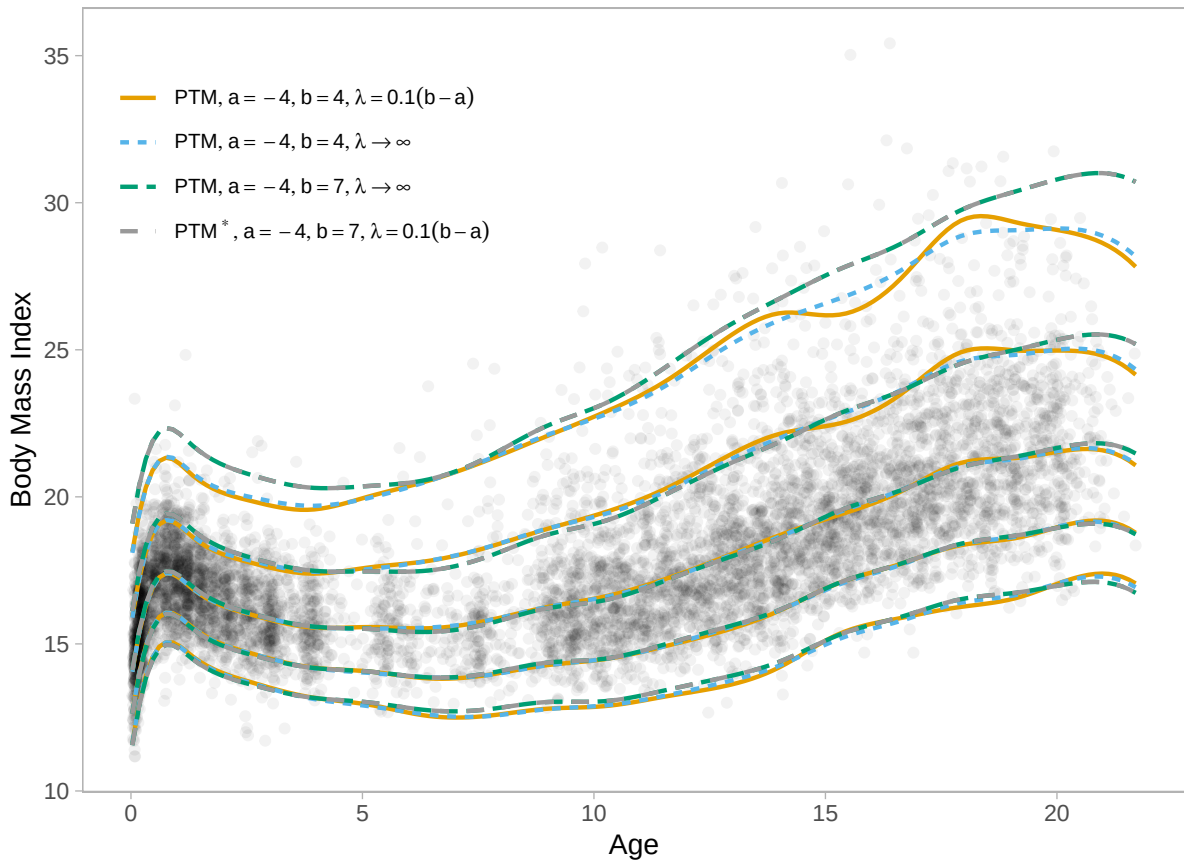
Quantile curves with different PTM specifications
