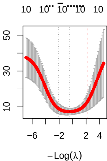
Mean-Squared Error
