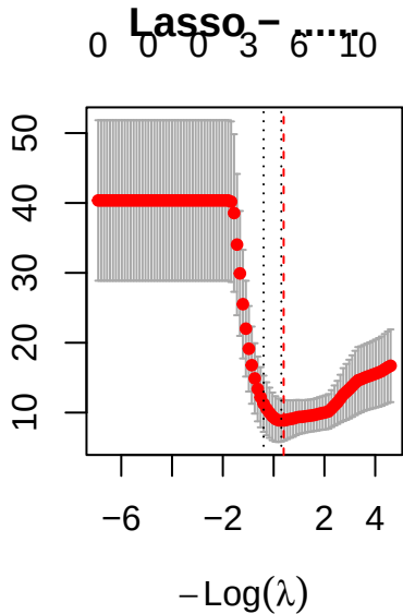
Mean-Squared Error
