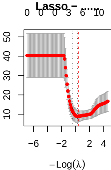
Mean-Squared Error
