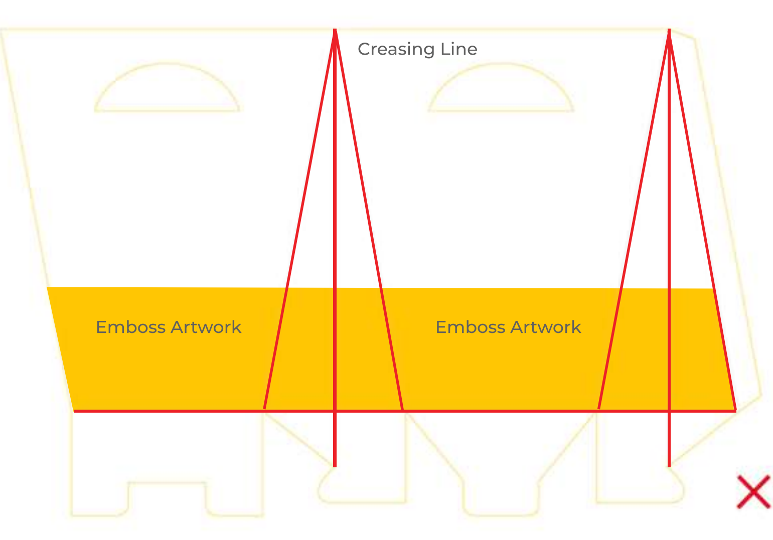
Embossing on a Packaging with Creasing Line demonstrated.
