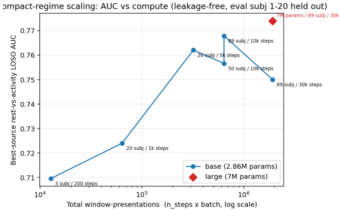
Fig. 1. Compact-regime scaling (leakage-free; eval subjects 1–20 held out from all pretraining). Best-source rest-vs-activity LOSO AUC vs. total window-presentations ( N_{\text{steps}} \times \text{batch} , log axis). The base 2.86M model rises then plateaus near 0.76 AUC; the 7M-parameter model (diamond) sits above the plateau at matched data and compute, indicating the base-model plateau reflects model capacity rather than a hard data limit.
