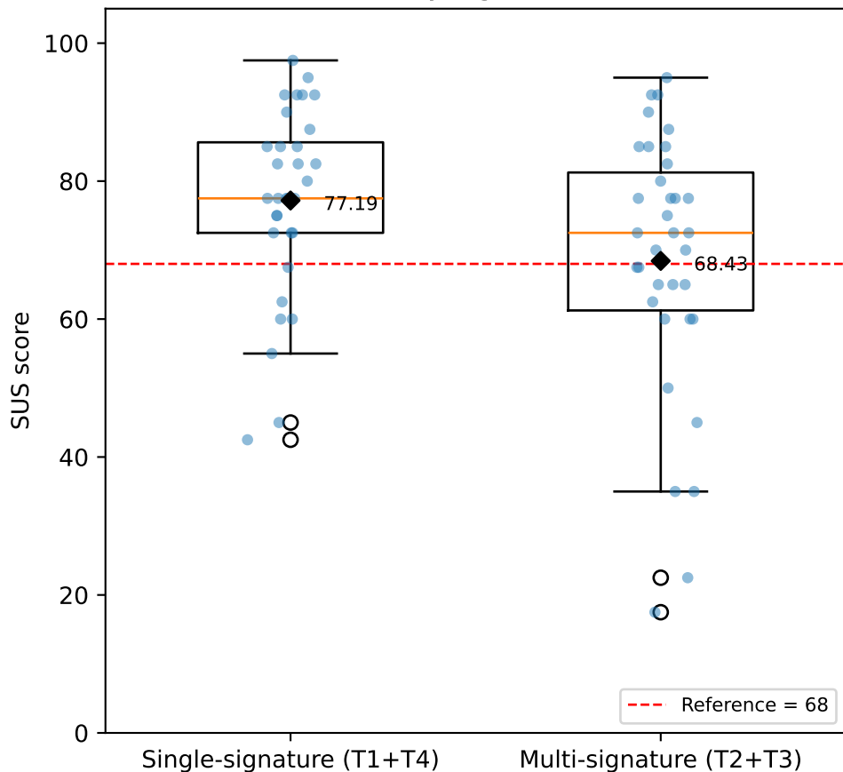
SUS scores by signature scheme
