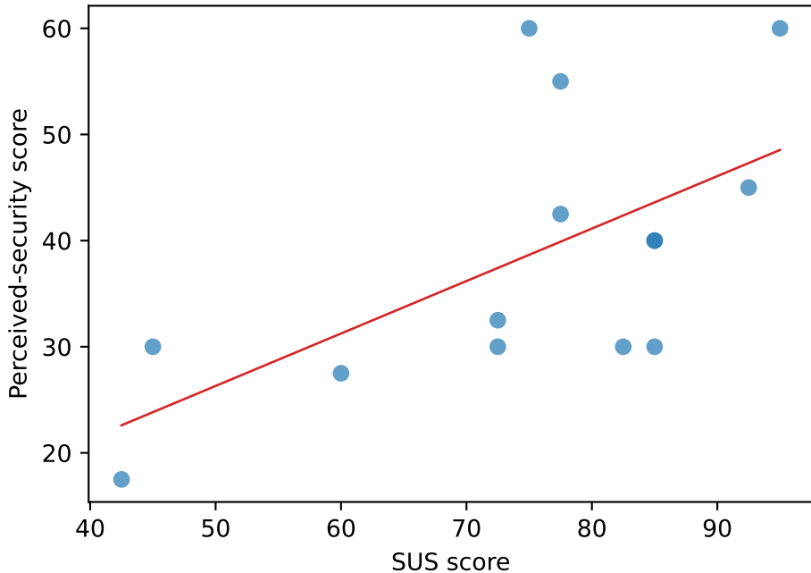
Treatment 1 - Mobile Device Only Spearman rho = 0.61, p = 0.0215
