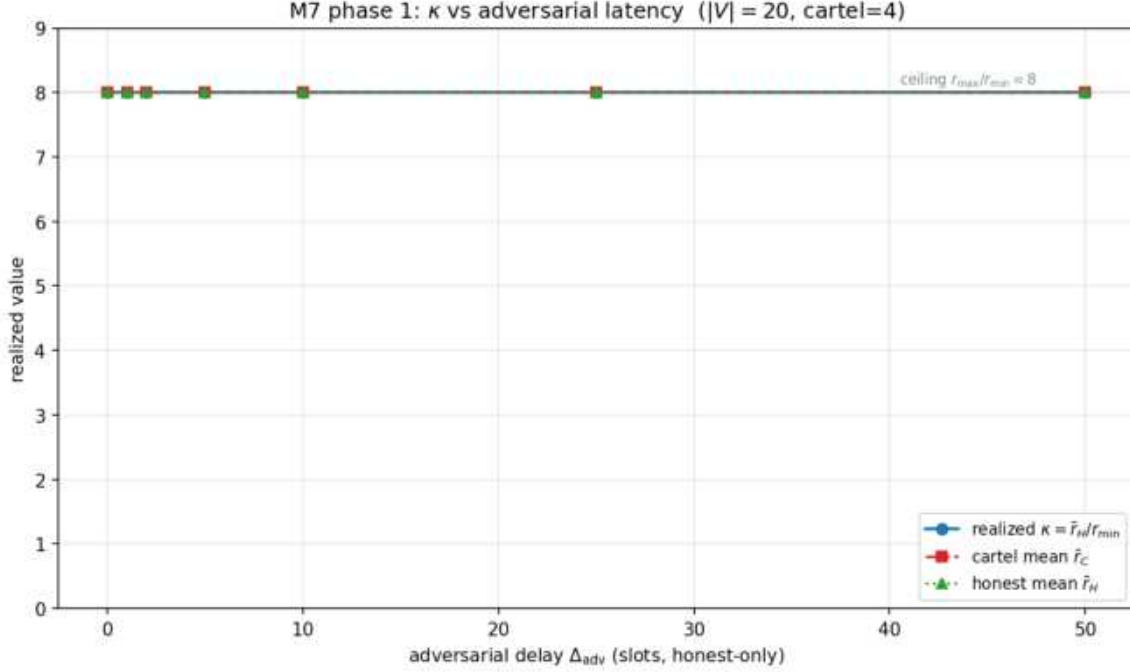
Figure 5: Realized \kappa across adversarial-latency settings. The x-axis is the cartel-vs-honest delivery delay \Delta_{adv} (slots); the y-axis is realized \kappa = \bar{r}_H/\bar{r}_{min} at steady state. The simulator’s per-validator delivery queue preserves the §4.3 voter-share semantics under arbitrary delay: late honest votes still contribute their per-block share, so \kappa stays at the r_{max}/r_{min} = 8 ceiling regardless of \Delta_{adv} . This is the simulator’s empirical statement; the analytical “BFT-bound collapse” regime is outside this single-chain model and is covered by the §5.2 inheritance argument. Generated by prototypes/poua-sim/scripts/run_adversarial_latency.py .
