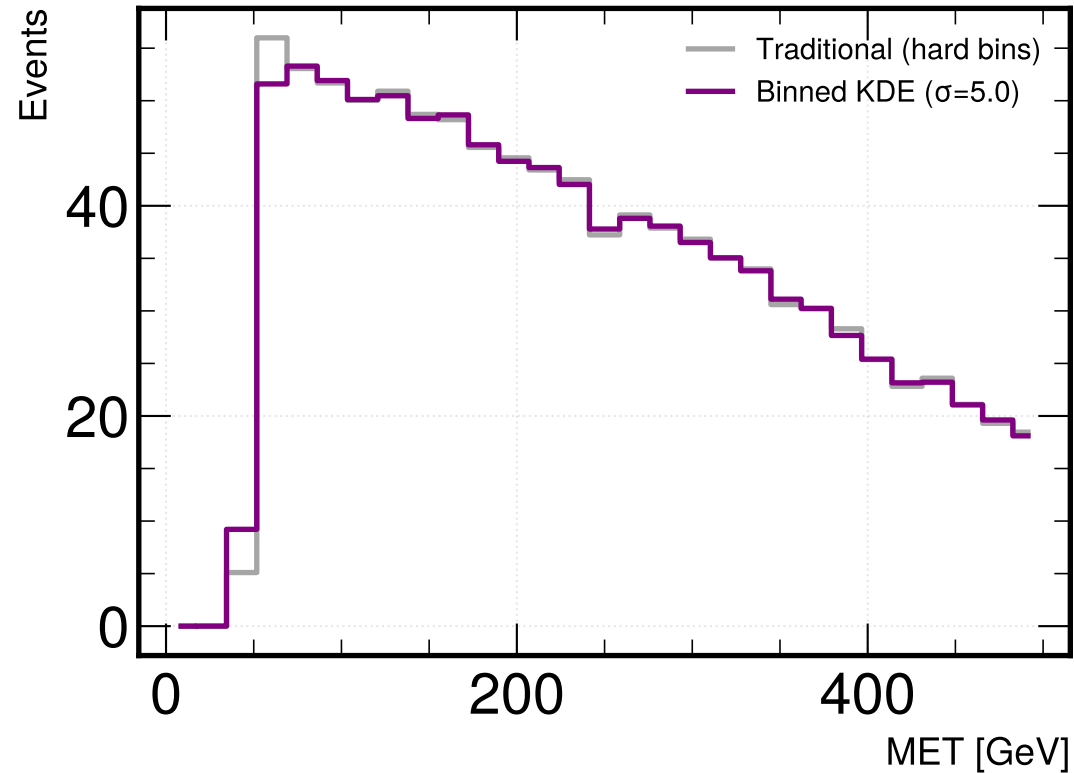
Bandwidth = 5.0 GeV
