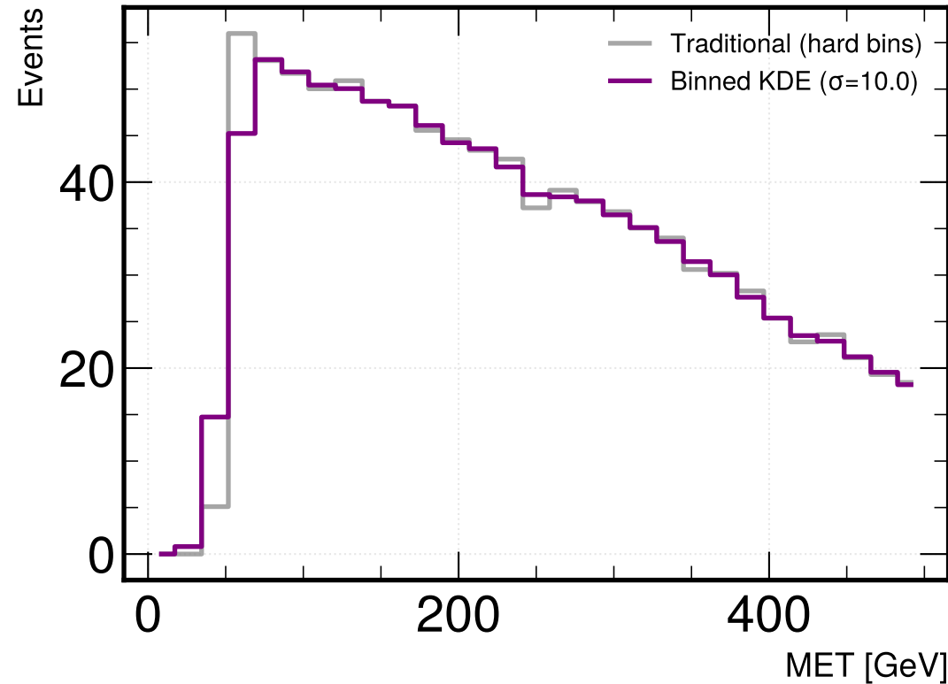
Bandwidth = 10.0 GeV
