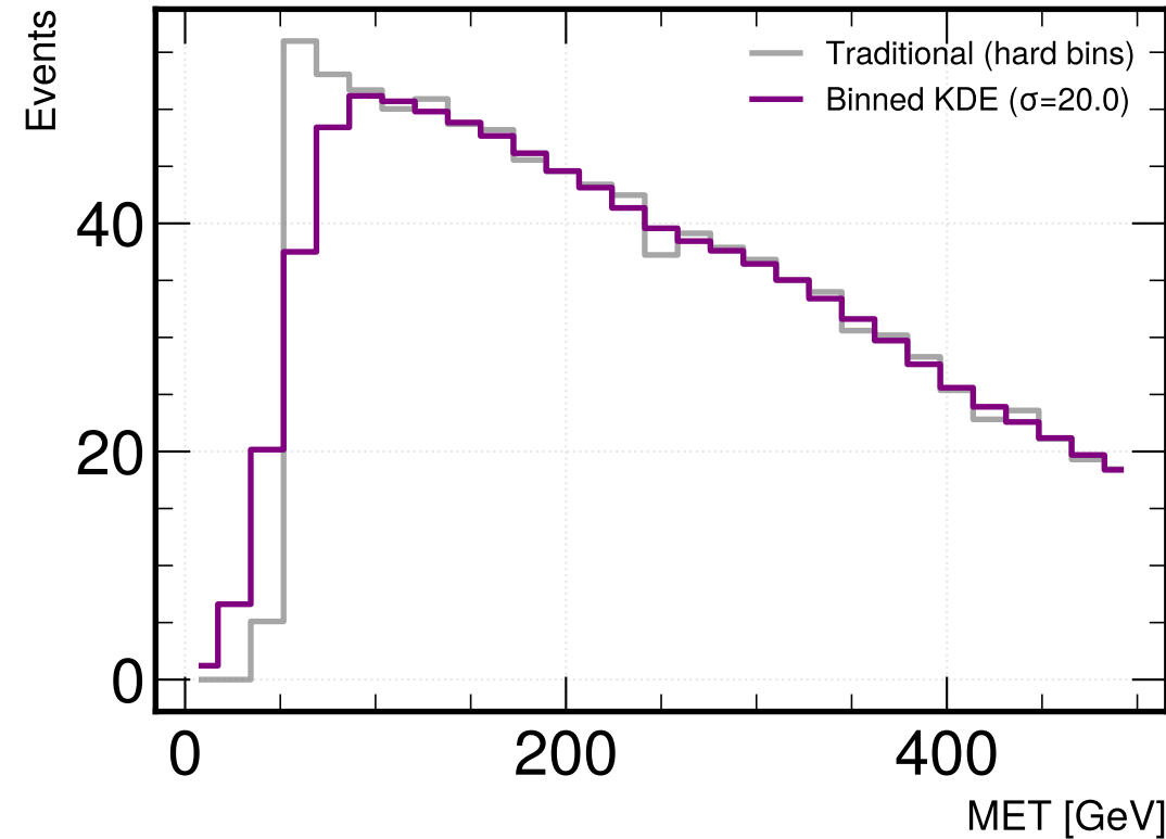
Bandwidth = 20.0 GeV
