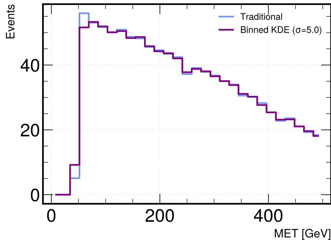
Bandwidth = 5.0 GeV
