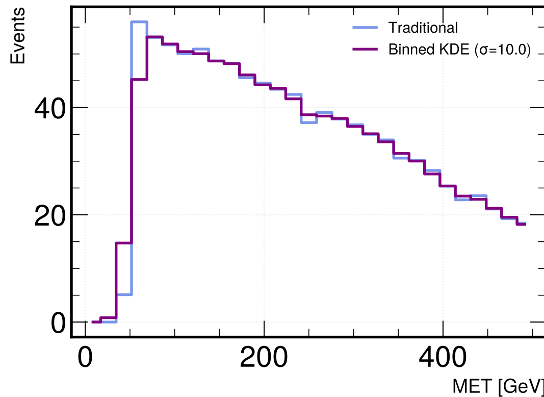
Bandwidth = 10.0 GeV
