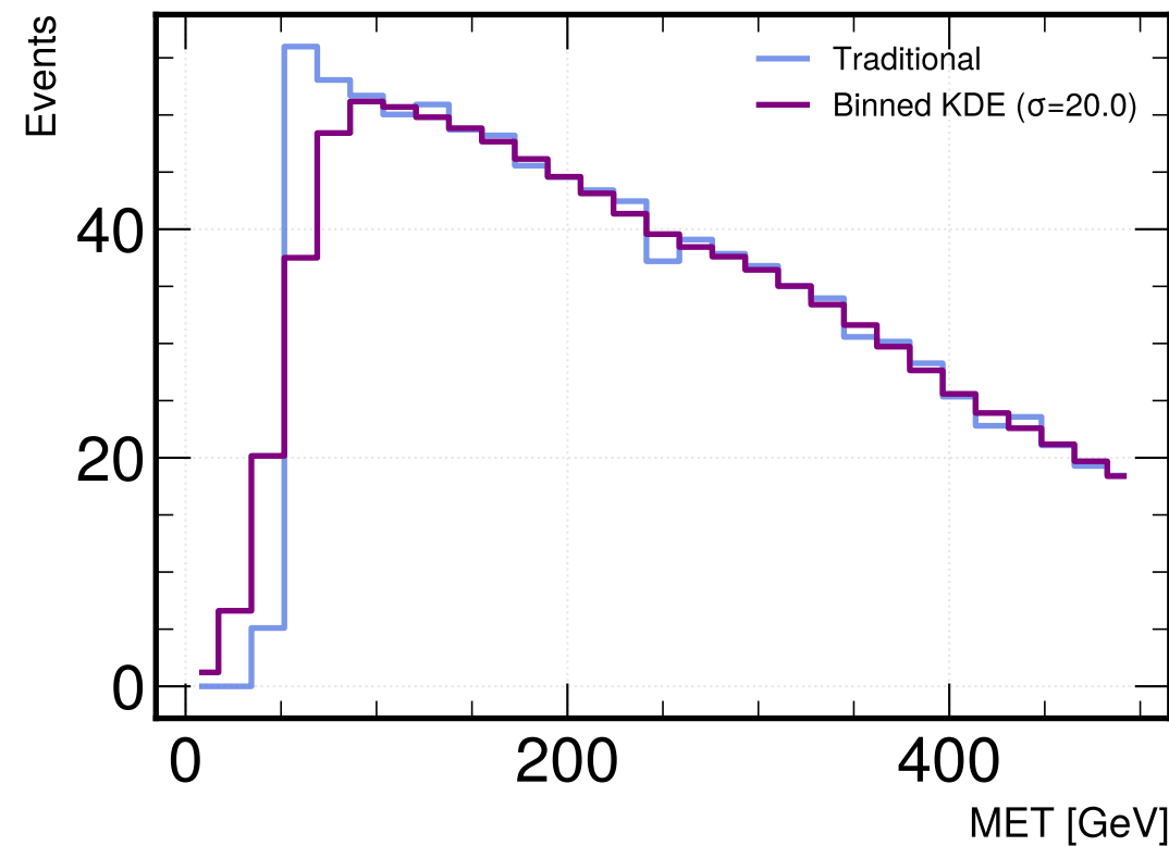
Bandwidth = 20.0 GeV
