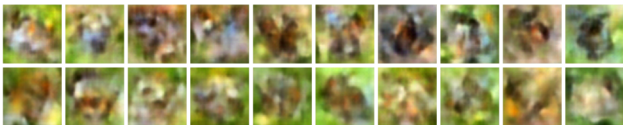
cVAE (c/mse)
