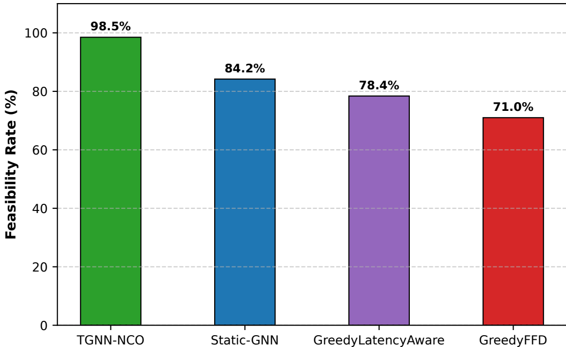
In-Distribution Feasibility Comparison
