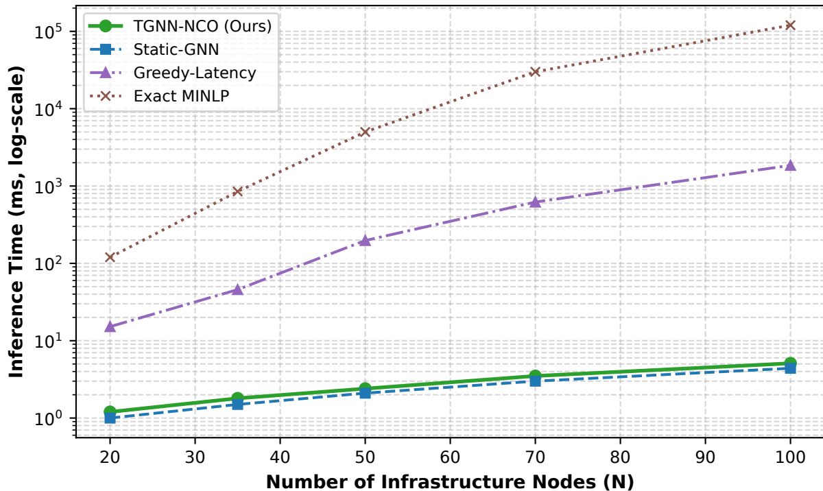
OOD Scalability: Inference Time vs Node Count
