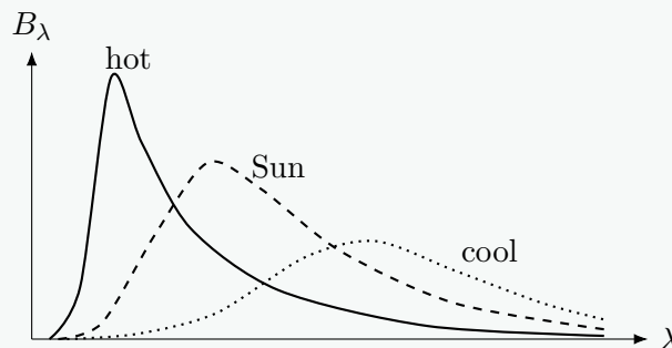
Figure 2: Qualitative black-body spectra.
