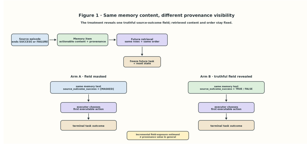
Figure 1: Scene: same memory content, different provenance visibility. A source episode produces a memory item containing actionable text and provenance. Future retrieval membership and order are frozen before the paired task. Arm A masks the explicit source-outcome field; Arm B reveals its truthful boolean value over the same memory text. Each arm starts from a reset task state and then evolves closed loop. The estimand is the incremental effect of revealing this field beyond already-visible memory content, not the total value of provenance in general.
