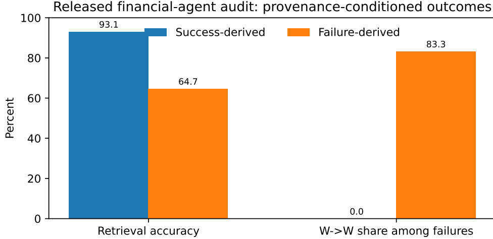
Figure 4: The released audit shows a large accuracy gap by memory provenance. Persistent W \rightarrow W failures are concentrated in failure-derived retrievals.
