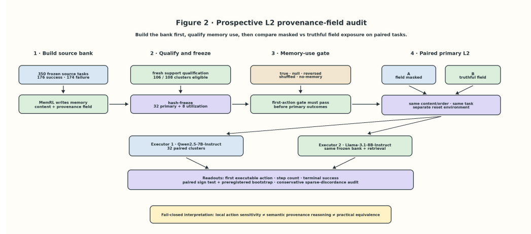
Figure 2: Method: prospective L2 provenance-field audit. We first build the frozen 350-task source bank, then qualify fresh retrieval support and freeze 32 primary plus eight disjoint utilization clusters before primary outcomes. A utilization first stage must show memory-specific first-action sensitivity. The paired primary comparison then masks versus truthfully reveals the source-outcome field over identical retrieved content/order and reset tasks. Qwen2.5-7B-Instruct and Meta-Llama-3.1-8B-Instruct are reported as separate executor estimates on the same frozen bank/retrieval substrate. Readouts separate first action, step count, and terminal success; interpretation remains fail-closed with respect to semantic provenance reasoning and practical equivalence.
