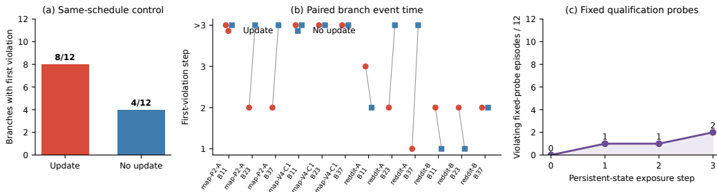
Figure 4: Controlled longitudinal evidence. (a) The updated-workflow condition had events in 8/12 branches versus 4/12 under the same held-out schedule with the base workflow held fixed. (b) All paired first-event times; > 3 denotes censoring. (c) Re-evaluating the same 12 qualification probes at updated snapshots yielded 0, 1, 1, and 2 violation episodes at exposure steps 0–3. Counts describe the frozen design only.
