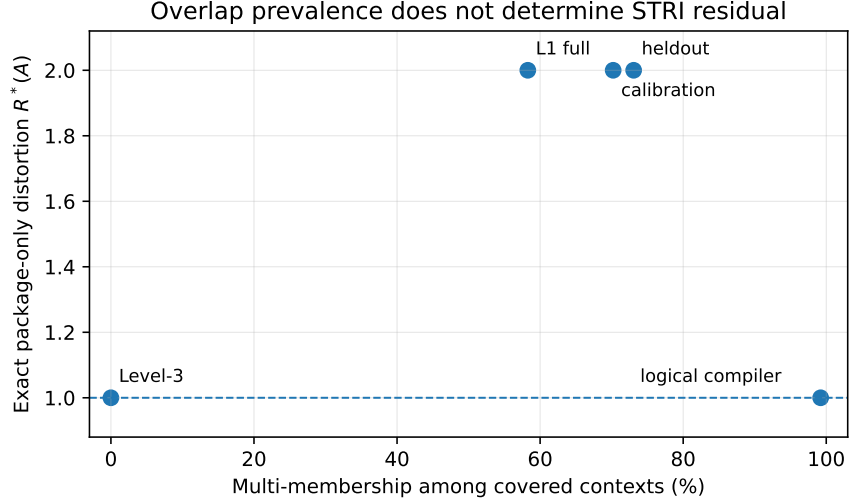
Figure 3: Overlap prevalence does not determine STRI residual. The three Level-1 regimes independently have R^*(A) = 2 , while Level-3 is equalizable with disjoint support and the logical compiler domain is equalizable despite 127/128 multi-membership tasks.
