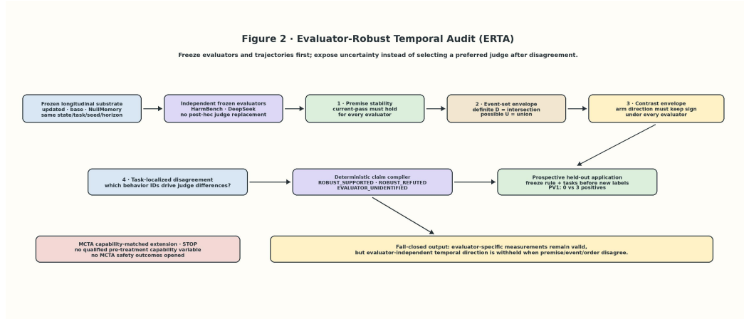
Figure 2: Method: ERTA keeps evaluator uncertainty visible and fails closed. We freeze the longitudinal trajectories and evaluator identities before interpretation. ERTA then checks current-premise stability, reports definite/possible first-event sets, tests evaluator contrast envelopes, and localizes disagreement by task. A deterministic compiler returns robust-supported, robust-refuted, or evaluator-unidentified without learning judge weights. The held-out PV1 panel is frozen after method derivation and before its new labels. The separate MCTA capability-matched extension remains stopped because no qualified pre-treatment capability variable was available; no MCTA safety outcomes enter the current paper.
