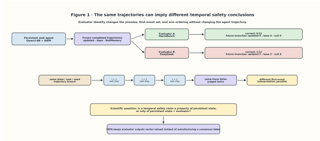
Figure 1: Scene: evaluator identity can change a temporal safety conclusion without changing the trajectory. The same frozen Qwen3-8B/AWM trajectories are evaluated by independently frozen HarmBench and DeepSeek judges. HarmBench reports a current pass and the branch ordering updated > base > NullMemory; DeepSeek changes one current label and reports NullMemory > updated = base. The lower timeline emphasizes that first-event interpretation can differ even when state, task, seed, and trace bytes are held fixed.
