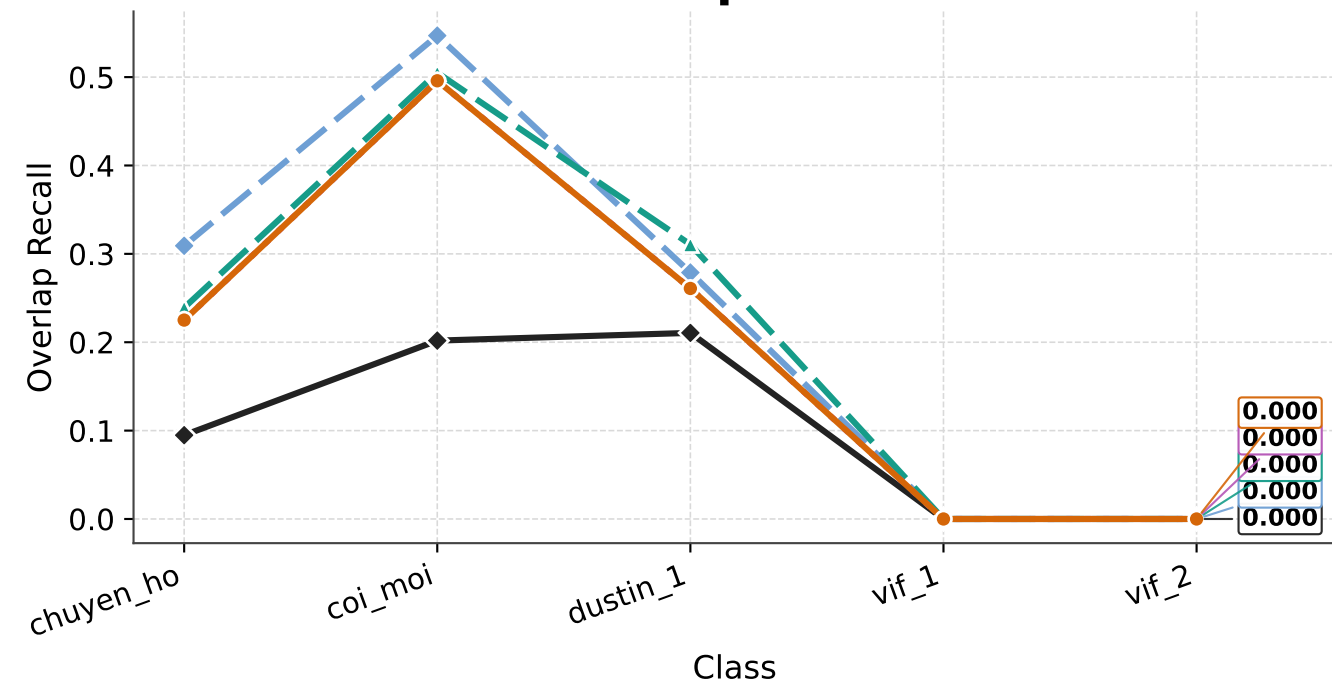
Predicted Segments
