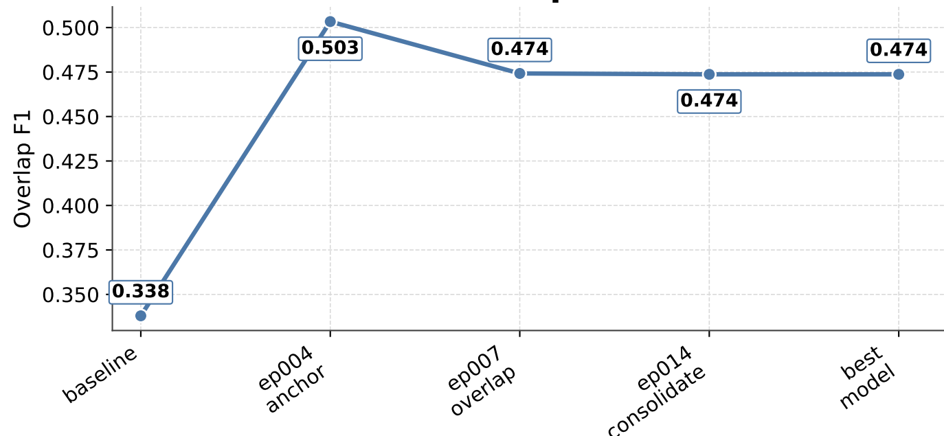
Overlap F1
