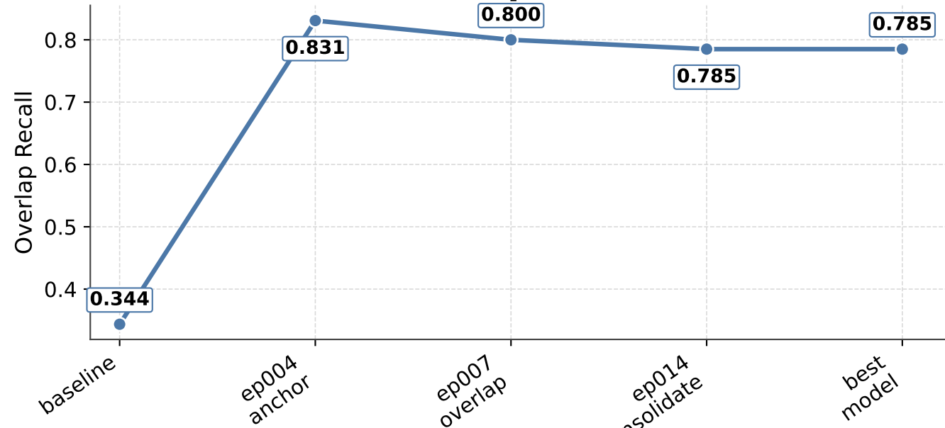
Predicted Segments
