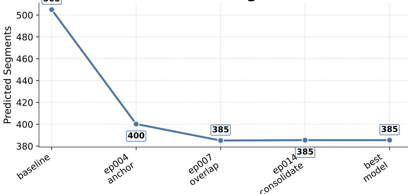
Predicted Segments
