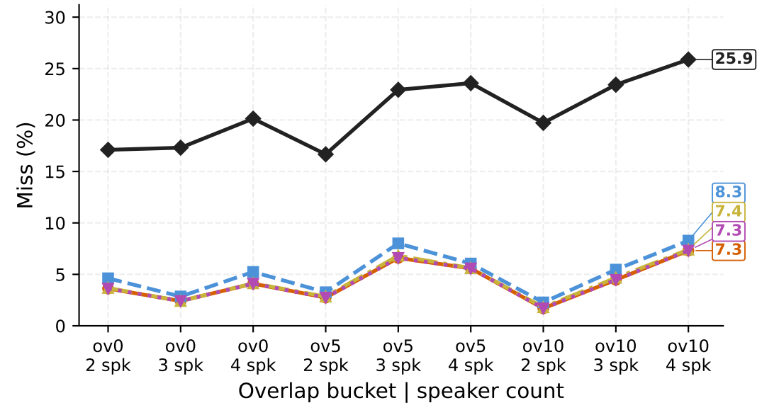
Miss (%)
