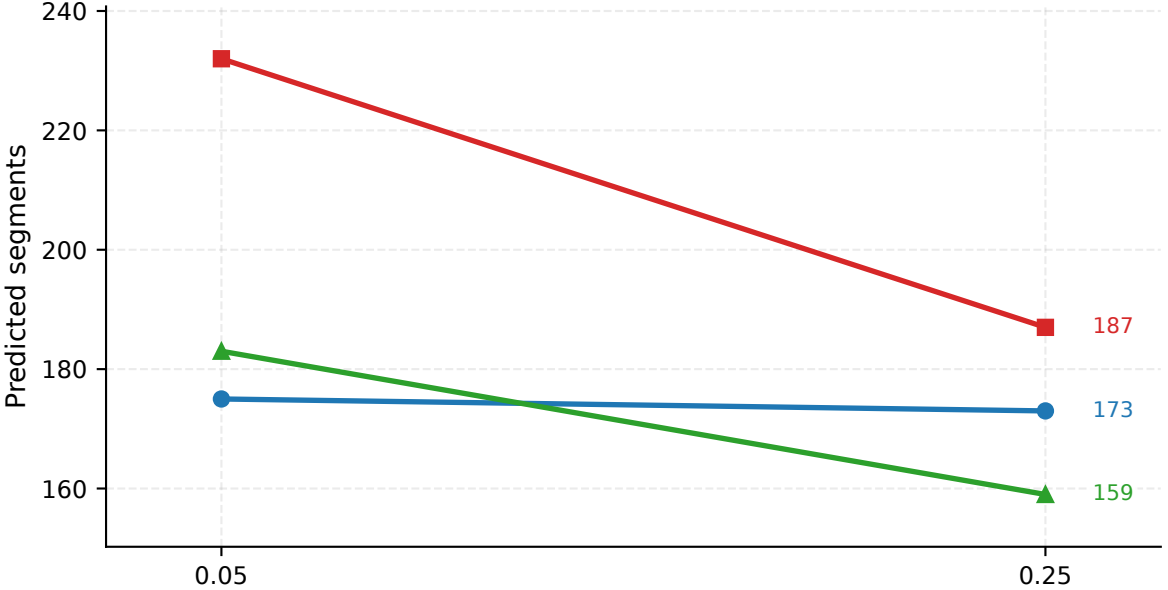
Predicted segments
