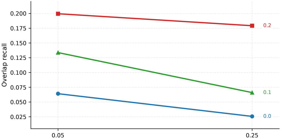
Predicted segments
