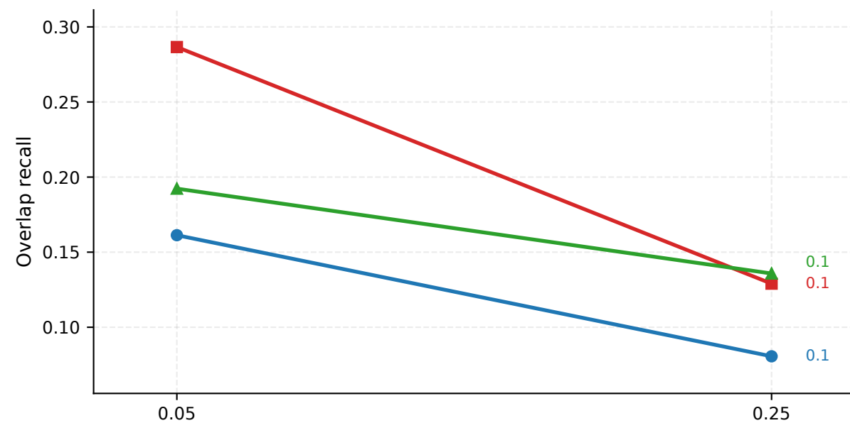
Predicted segments
