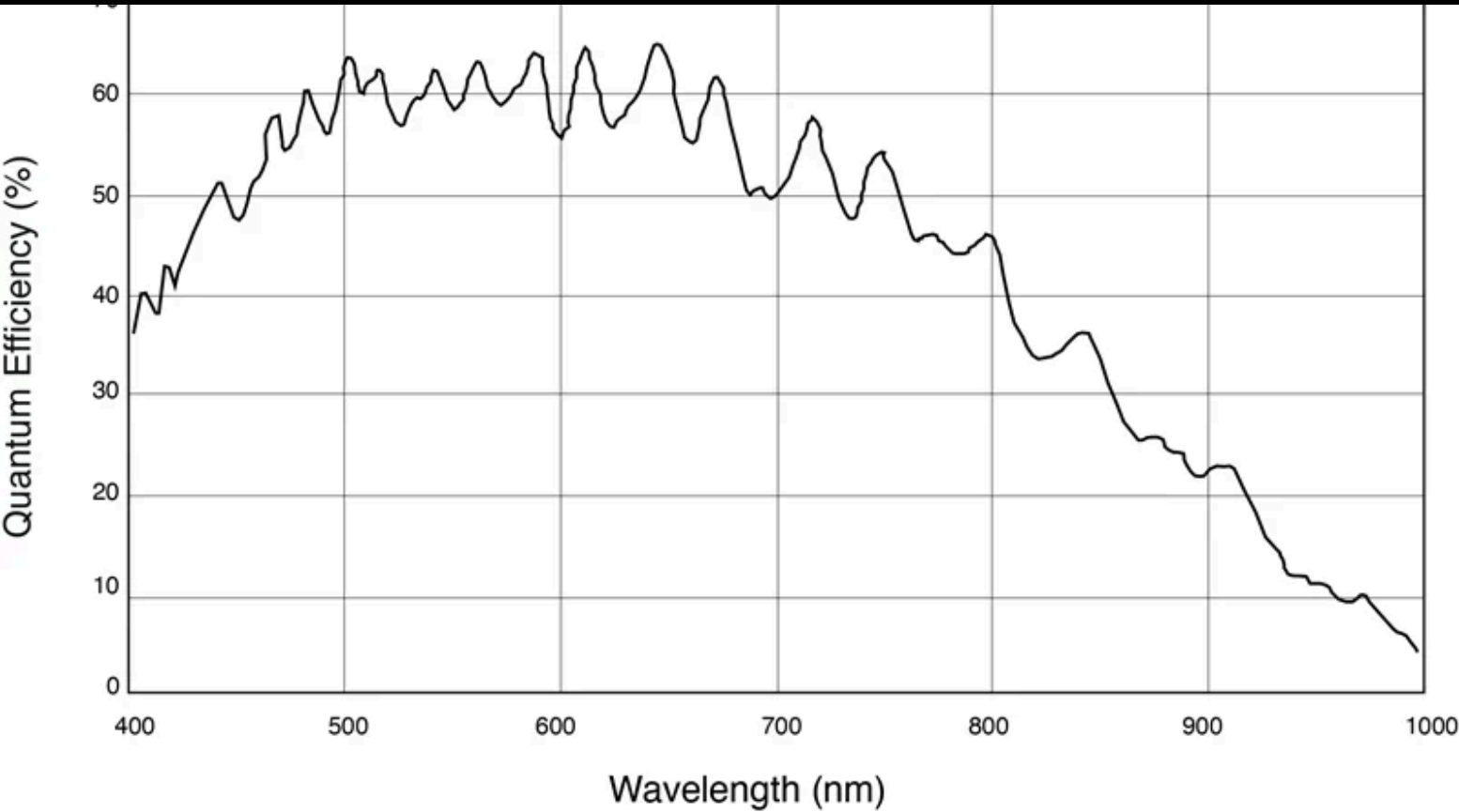
MT9P031 Sensor QE Curve
