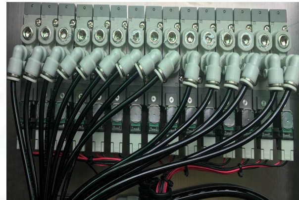
solenoid valve
