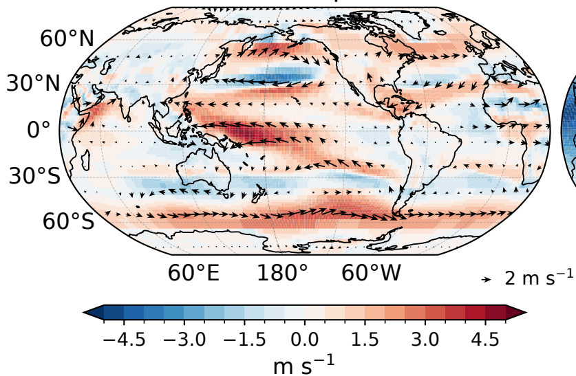
(c) 850 hPa Wind: Speed & Vectors
