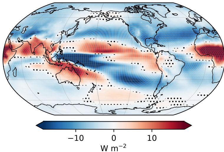
(h) Net radiation — TOA
