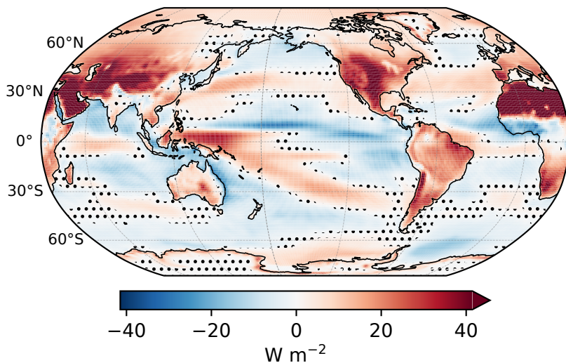
(e) Longwave — Surface
