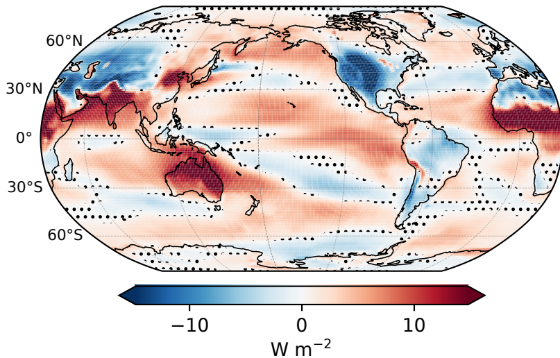
(g) Sensible heat flux — Surface
