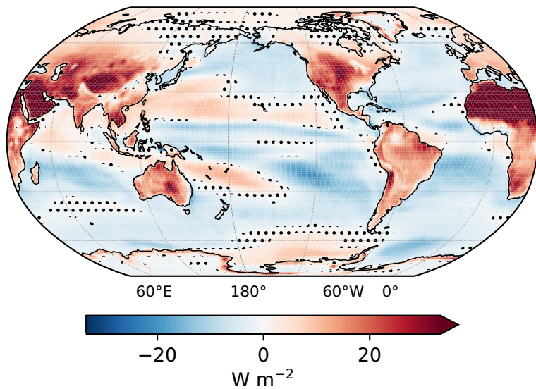
(h) Net radiation — TOA
