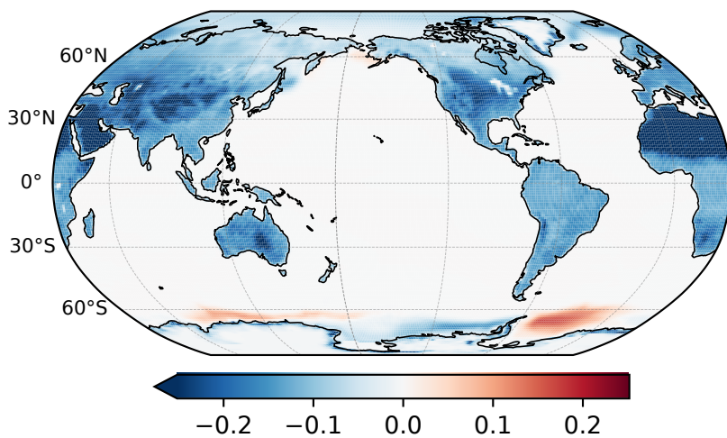
(c) Shortwave — Surface
