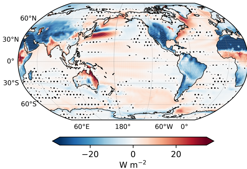
(g) Sensible heat flux — Surface
