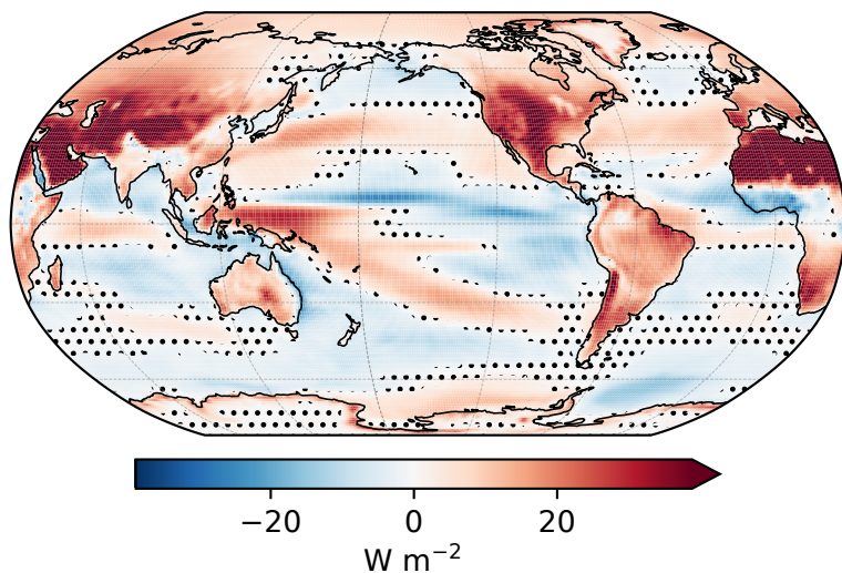
(f) Longwave — TOA
